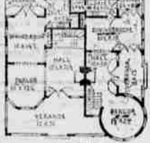
FIRST FLOOR.
