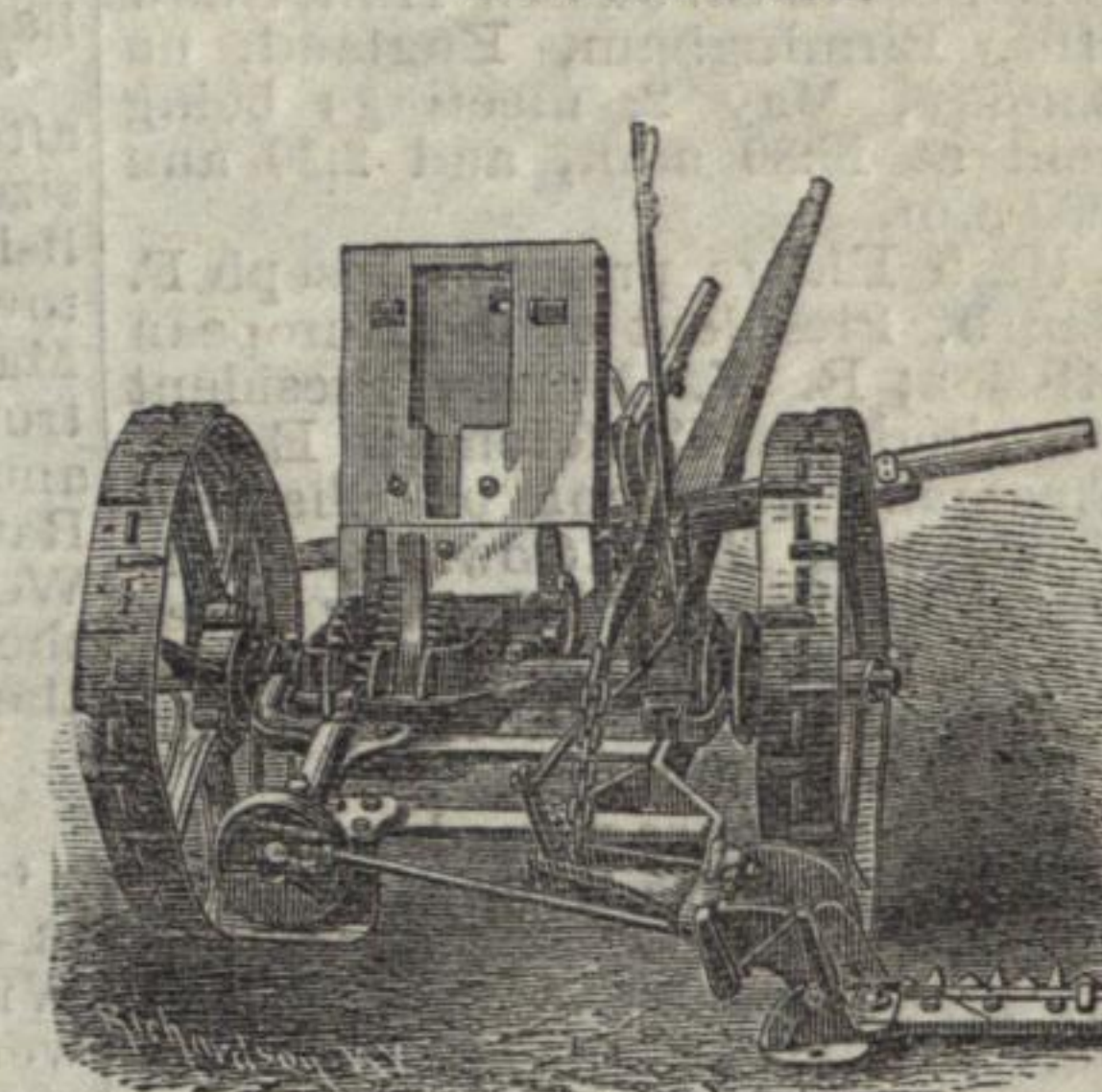
Showing Gearing.
