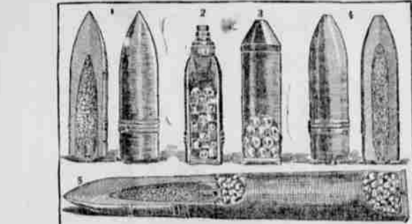
SECTIONAL VIEW OF AMMUNITION FOR RAPID-FIRE GUNS. THIS WILL BE MORE DAMAGING THAN THE BULLET.
